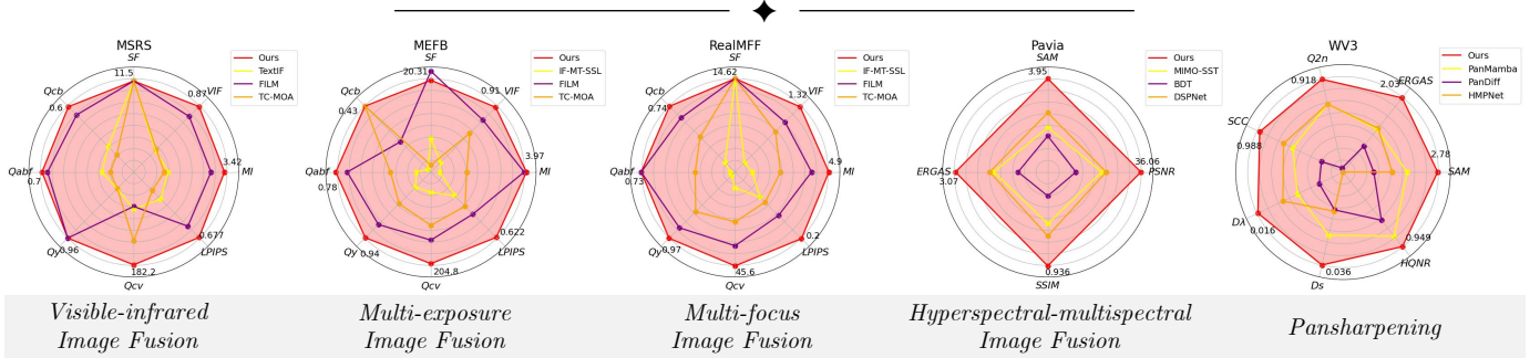
Fig. 1: Performance assessment on several image fusion tasks comparing with state-of-the-art methods.
