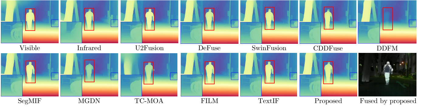
Fig. 11: Monocular depth estimation results by using Depth Anything v2 [96]. Close-ups are depicted in the blue boxes.
