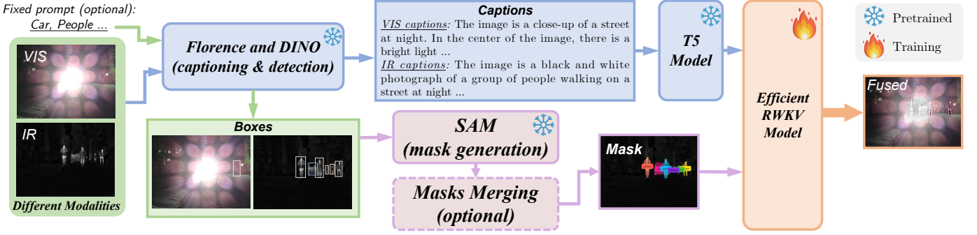
Fig. 4: An overview of the proposed semantic guidance branch. Image pairs of different modalities, optionally with fixed prompts, are input into pre-trained large multi-modal models (DINO [62]) to detect objects and generate captions (using Florence [32]). Object boxes are processed by SAM [33] to produce instance-level masks. A mask merging algorithm is used to merge objects in different masks. The encoded captions from the T5 [61] model, along with the mask, are then fed into the proposed RWKV model to guide fusion processes.
