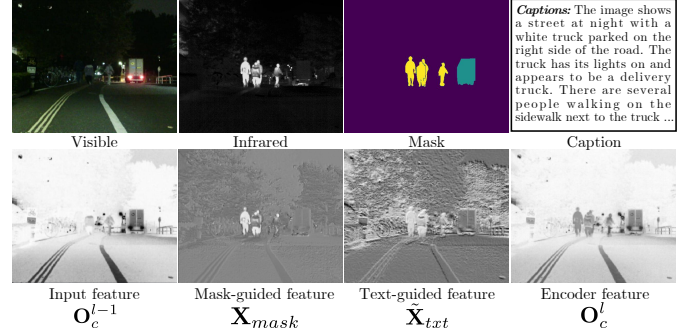
Fig. 6: Feature visualization for the MFM.
