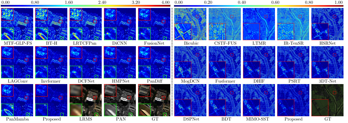
Fig. 9: Error maps with respect to the GT image for the compared approaches considering the pansharpening and the HMIF tasks. The left and right panels respectively showcase the error maps of “area 5” from the WV3 test set and “area 1” from the Chikusei ( \times 4 ) test set using a pseudo-color representation. Close-ups are depicted in the red and green boxes. PAN and LRMS stand for panchromatic and low resolution multispectral images, respectively.
