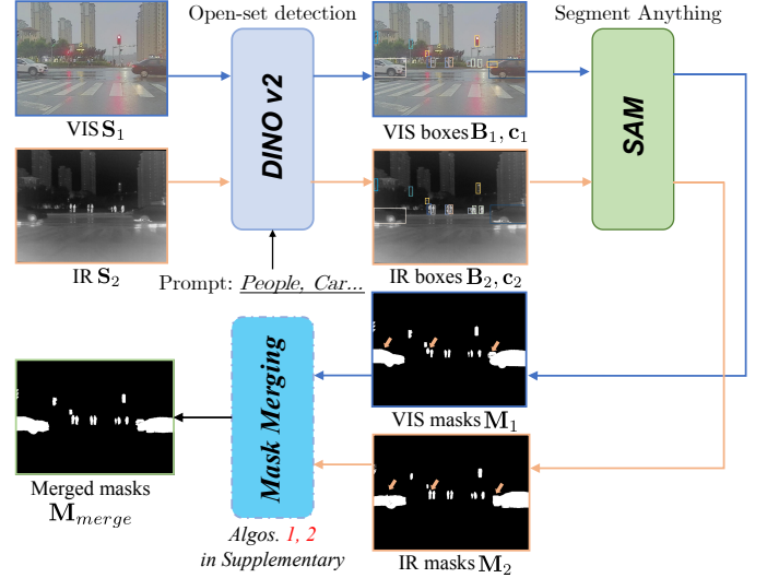
Fig. 7: An overview of mask segmentation and merging. Images from different modalities are fed into DINO and SAM to detect boxes and segment masks in an open-set manner. A novel mask merging algorithm is proposed. Technical details and symbol definitions are reported in Algos. I and II in Suppl. Sect. 3.
