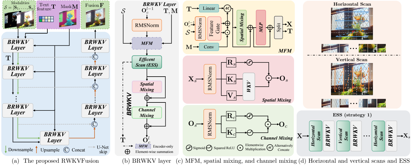
Fig. 5: Architecture of the proposed RWKV network. It relies upon a U-Net multi-scale framework, incorporating raw information from each modality, captions, and masks at various layers as conditions to guide the fusion process. Each BRWKV layer has four key components: i ) multimodal fusion module (MFM), ii ) efficient scanning strategy (ESS), iii ) spatial mixing, and iv ) channel mixing. Note that text feature \mathbf{T} is input from the previous BRWKV encoder layer, but mask \mathbf{M} is a condition injected into each encoder layer.
