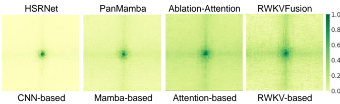
Fig. 10: Effective receptive fields (ERF) for architectures based on different operators (i.e., convolution, Mamba, attention, and RWKV) are visualized.
