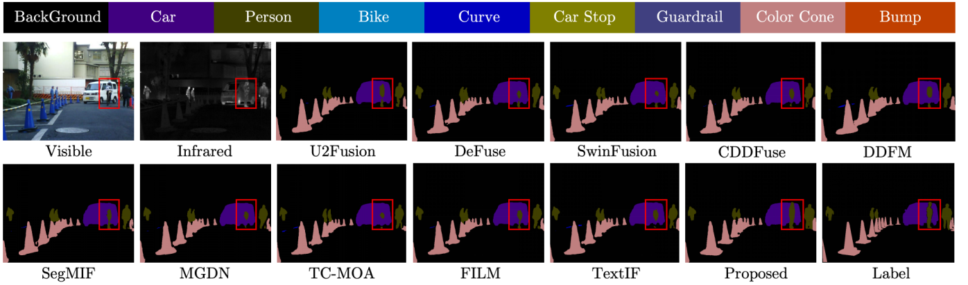
Fig. 12: Semantic segmentation results using Segformer [99] on images fused by the proposed RWKV Fusion and compared with previous methods. Segformer was trained separately on the corresponding fused/GT image pairs, with all configurations held constant across experiments. Red boxes show segmented objects that cause mIoU differences.
