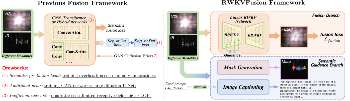
Fig. 3: Comparison between previously developed fusion frameworks and the proposed RWKVFusion. The main differences are as follows: i ) some of these frameworks incorporate additional tasks, such as segmentation [9], [15] and object detection [54], requiring semantic information, thus introducing training overhead and costly manual annotations; ii ) complex priors lead to the use of further networks [11] or a larger number of parameters and longer inference time [12], [13]; iii ) they exploit inefficient networks characterized by high computational demands, restricted receptive fields, and some other limitations [55], [56]. Our RWKVFusion introduces automatic open-set detection and mask generation to include semantic information to guide fusion processes without expensive annotation. VIS and IR stand for visible and infrared.
